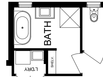
OPTION 3 EURO LAUNDRY & WC
