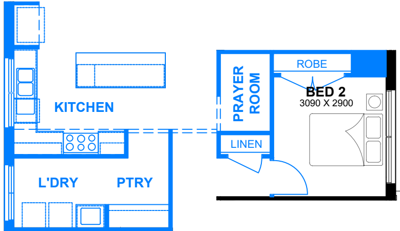
OPTION 2 PRAYER ROOM & ALTERNATIVE WIP
